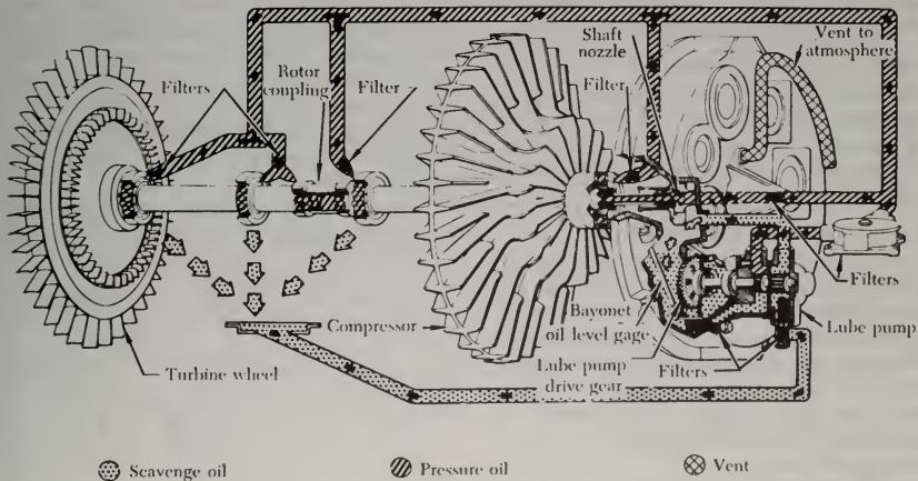
FIGURE 6-33. Turbojet engine wet-sump lubrication system.
